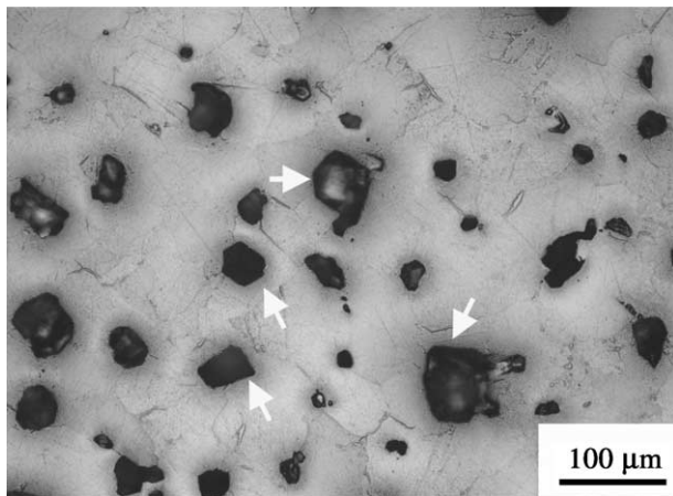
Fig. 5. Microstructure resulting from isothermal foaming at 903 °C for 58 h resulting in 11% total porosity and a relative open porosity ratio, F=0.05 . Examples of faceted pores are marked by arrows.
