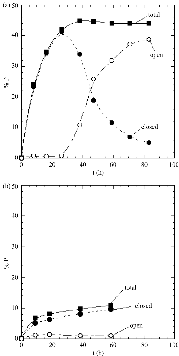
Fig. 2. Total, open and closed porosity as a function of time during (a) thermal cycling (830–980 °C) and (b) isothermal foaming (903 °C).
