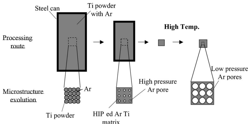
Fig. 1. Schematic of foaming process, where titanium powders are compacted by HIPing in the presence of argon and the resulting high-pressure argon bubbles then expand under low-pressure argon atmosphere at high temperature.
